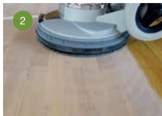
2 Abrade the surface using Bona Diamond Abrasive discs attached to the Bona FlexiSand
